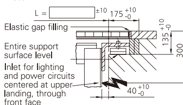
Detail Z
