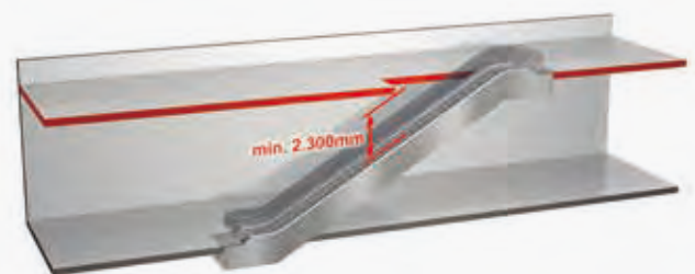
Overhead clearance
